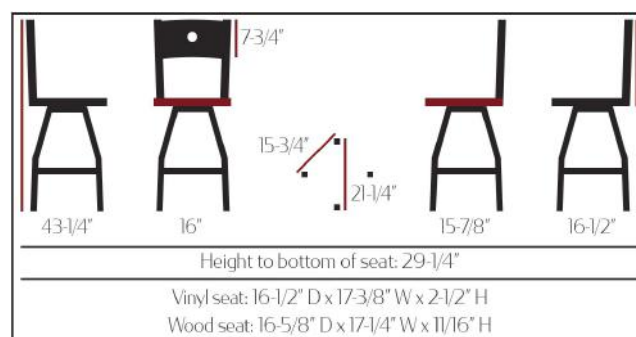
SL2150CCS-IS-B-WB SL2150CCS-IS-B-WB-BUC
